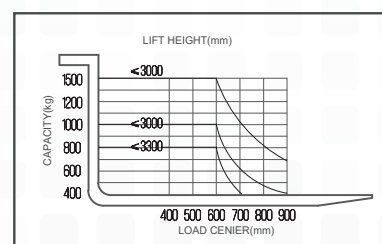
LOAD CHART
