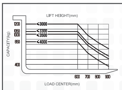
LOAD CHART
