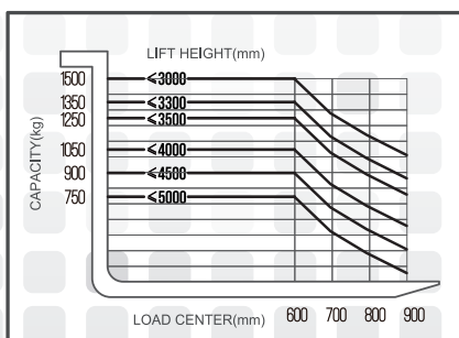
LOAD CHART
