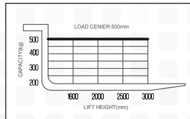
LOAD CHART
