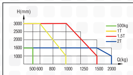
LOAD CHART
